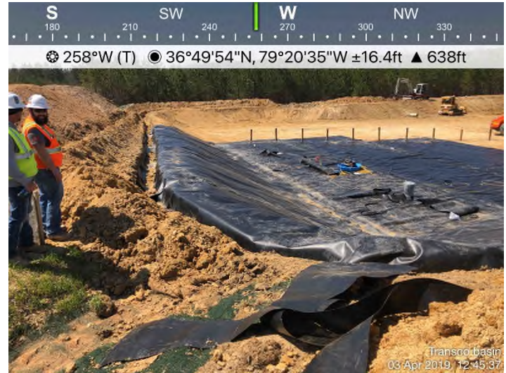
Fig. 8: Permanent Stormwater Pond – Emergency spillway.
