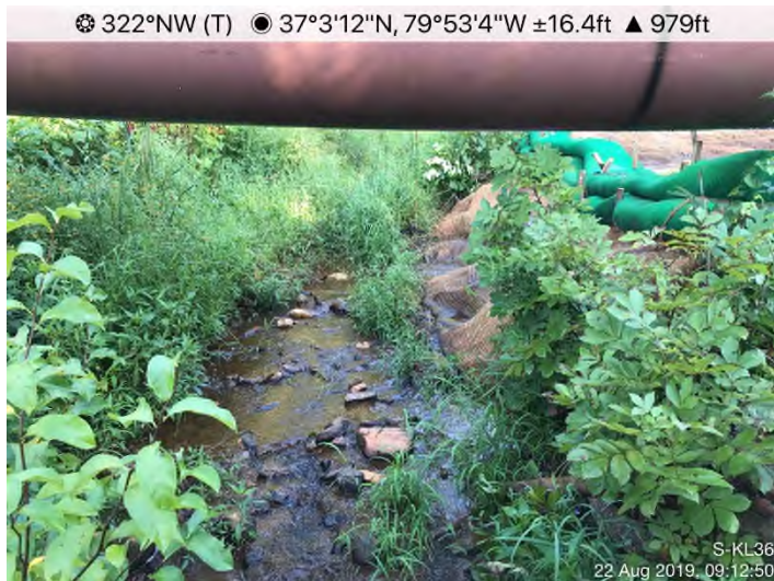
Fig. 3: STA 14019+91 – Area stabilized with erosion fabric, seed and straw.
