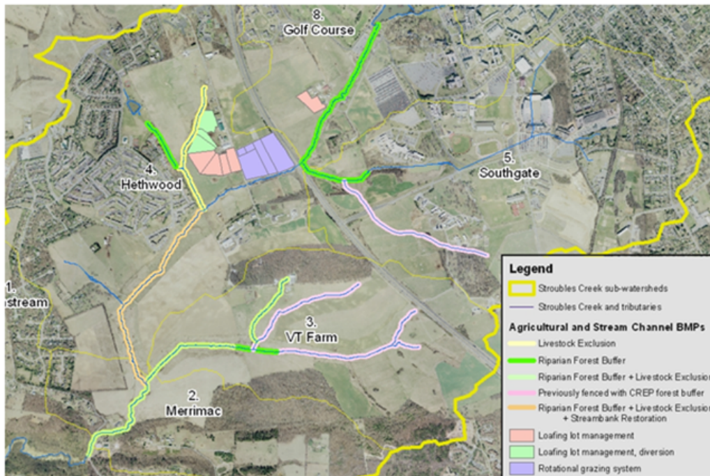
Figure 8.2. Example of agricultural and stream channel BMP targeting
