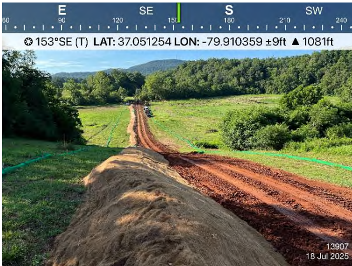
Fig. 3 STA 13907+00: Controls in place and functioning properly.
