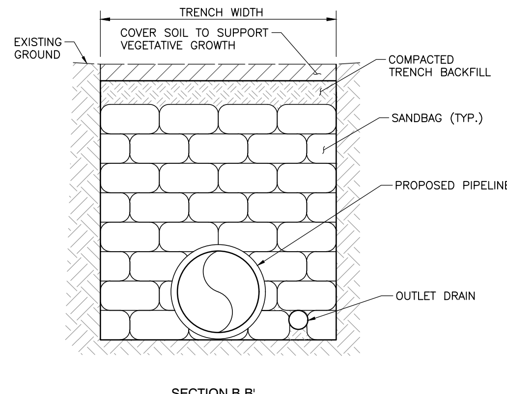
SECTION B-B'
