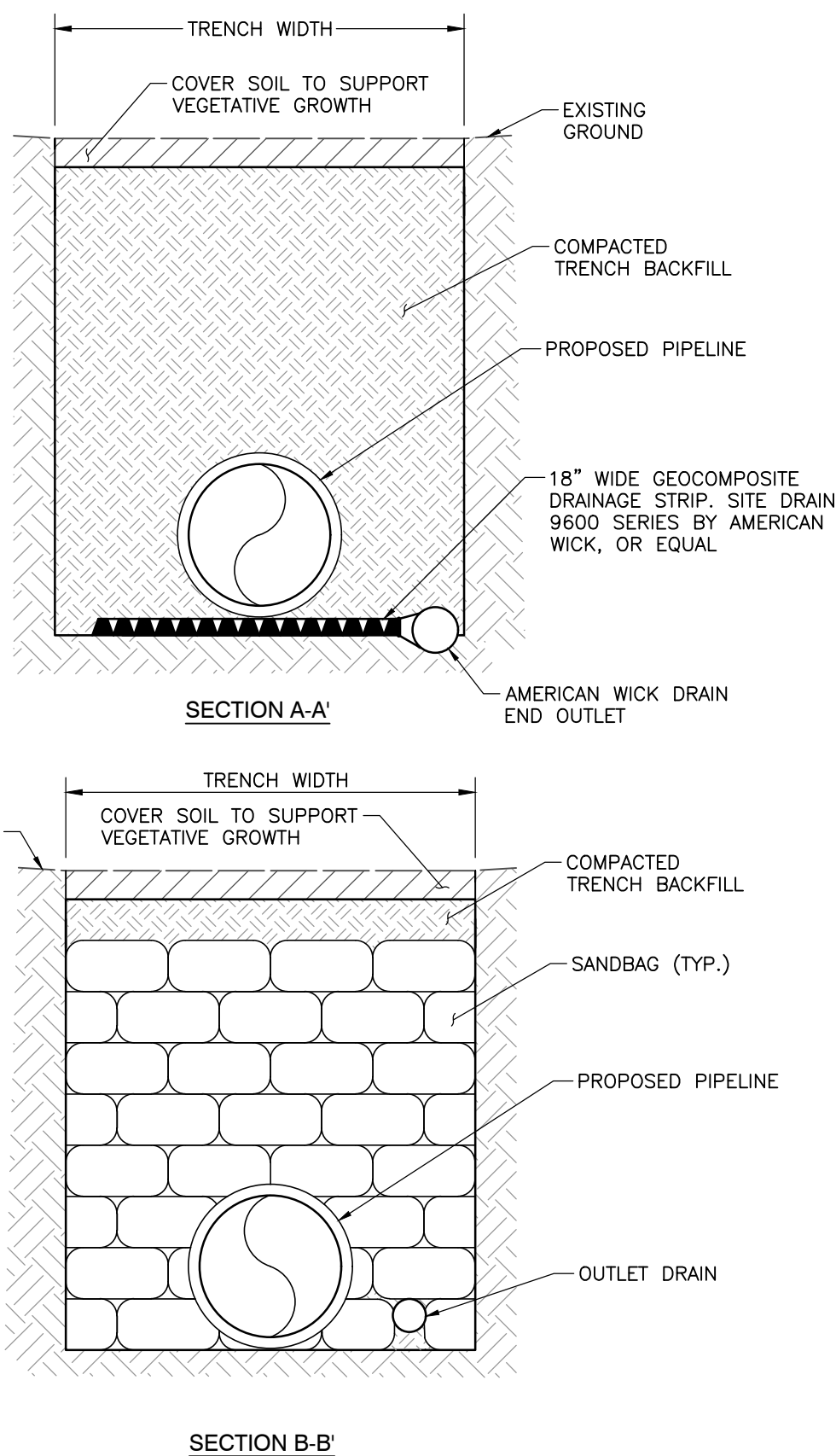
SECTION B-B'
