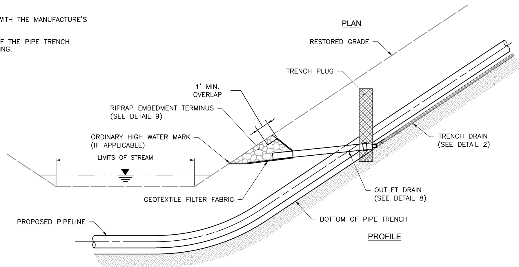
DETAIL 3 SLOPE TOE TRENCH DRAIN OUTLET NOT TO SCALE
