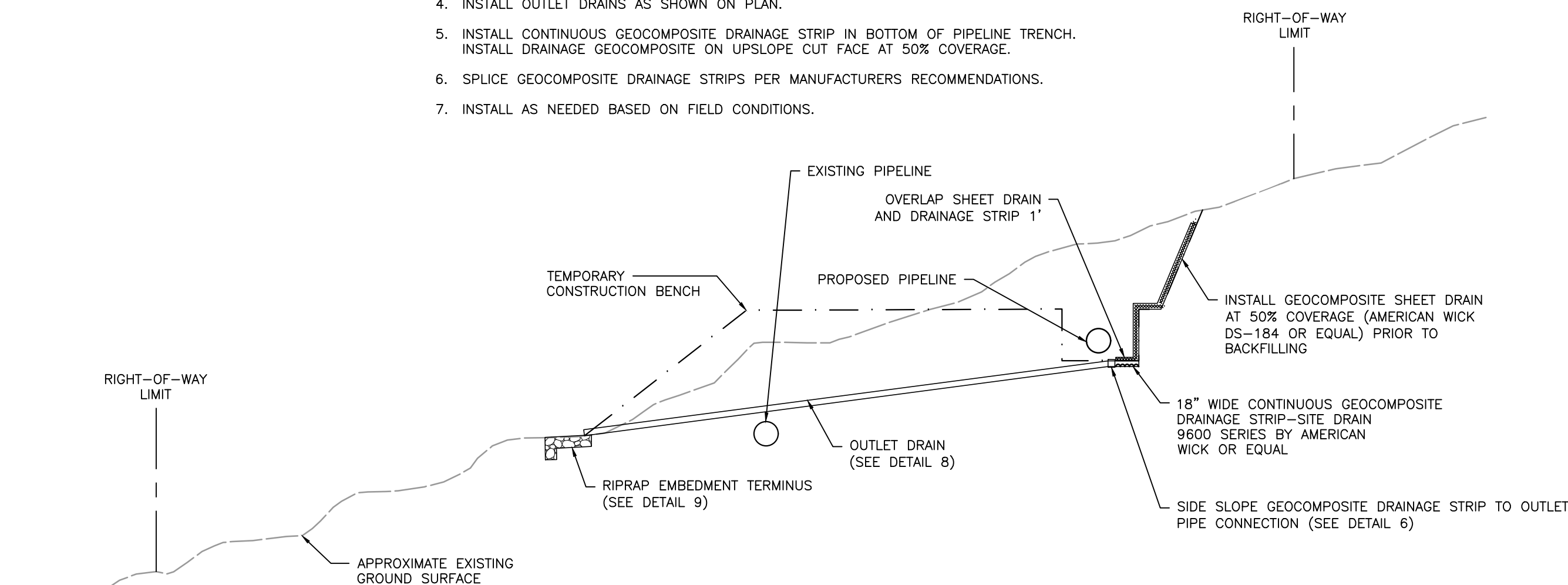
DETAIL 5 SIDE SLOPE TRENCH DRAIN NOT TO SCALE
