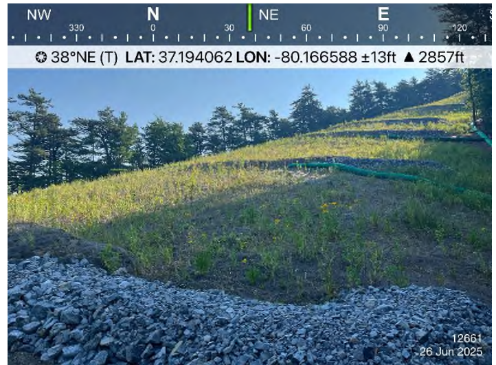
Fig. 4 STA 12661+00: Controls in place and functioning properly.
