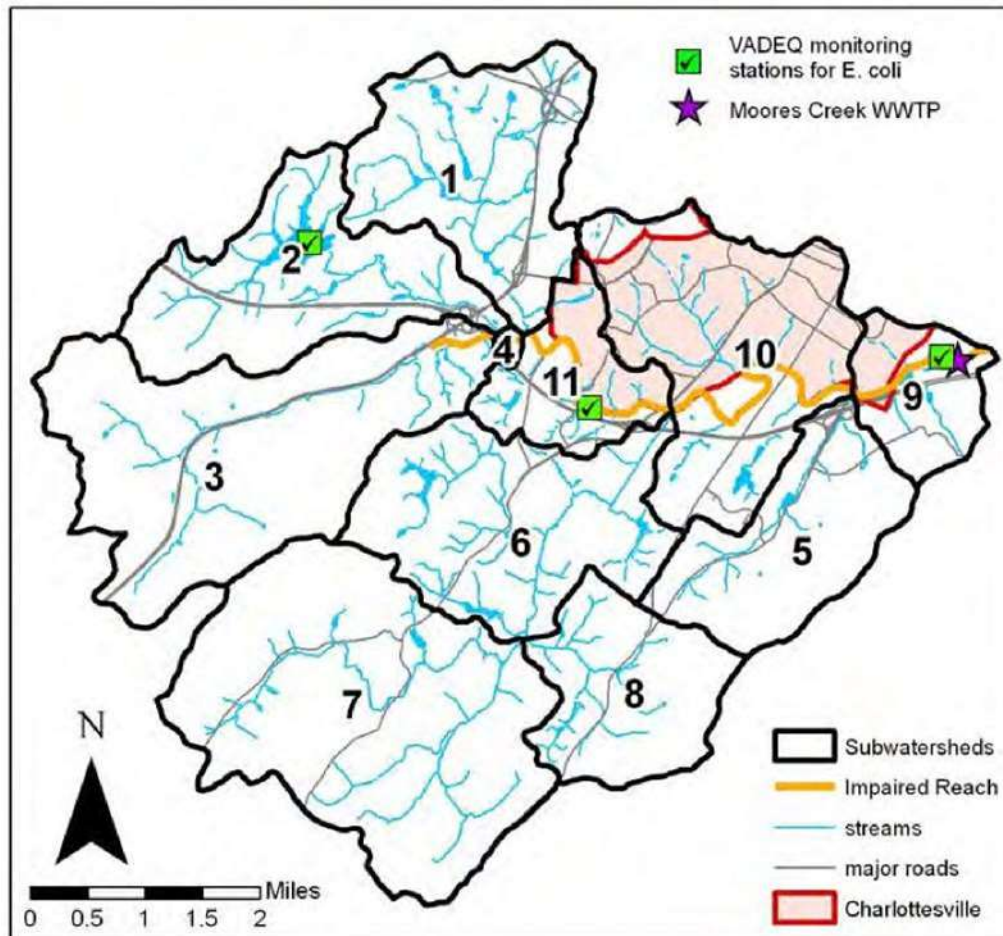
Figure 3.3 Monitoring stations in the Moores Creek watershed (DEQ, 2012).
