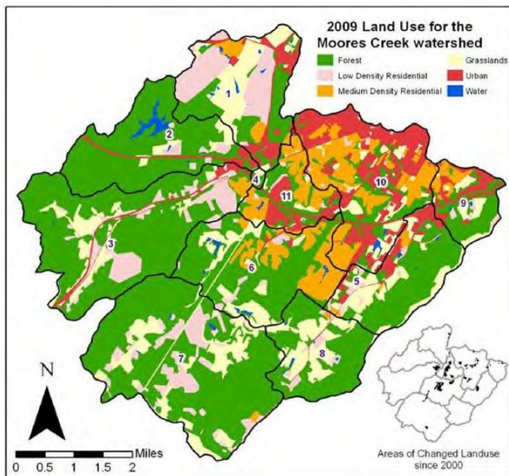
Figure 4.1 Land uses in the Moores Creek watershed.
