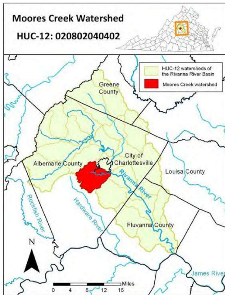
Figure 3.1 Location of the Moores Creek watershed.
