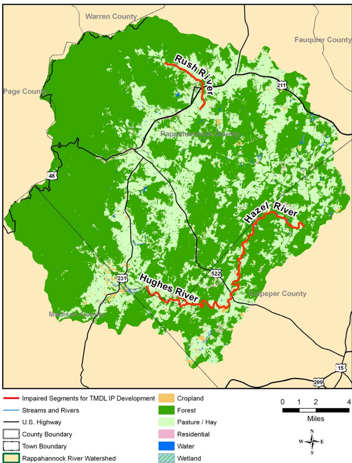
Figure 2. Land uses in the Upper Hazel River watershed.
