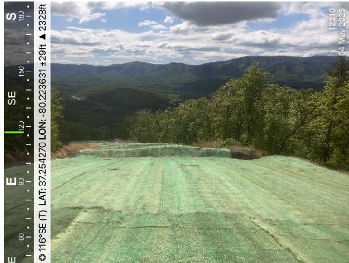
Figure 3: STA 12350+00 – Controls in place and functioning properly.
