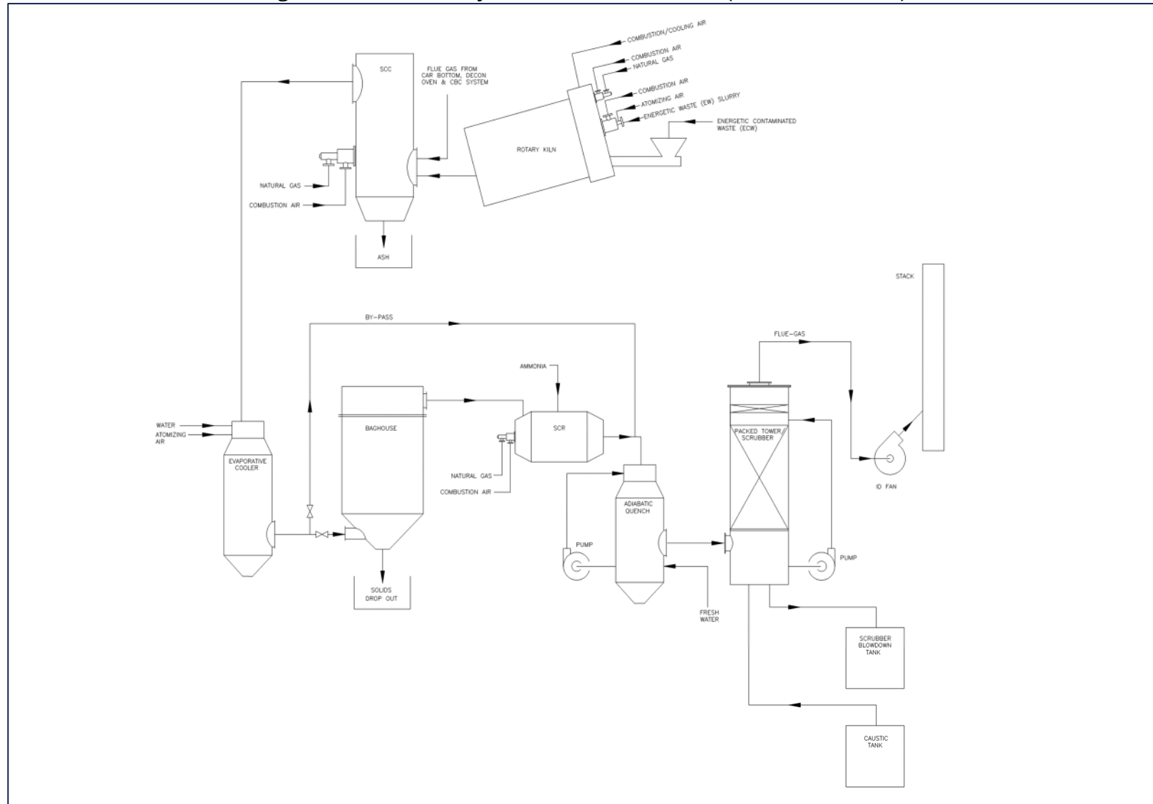
Figure II.Ea-5 - Kiln System Process Schematic (identical for each)
