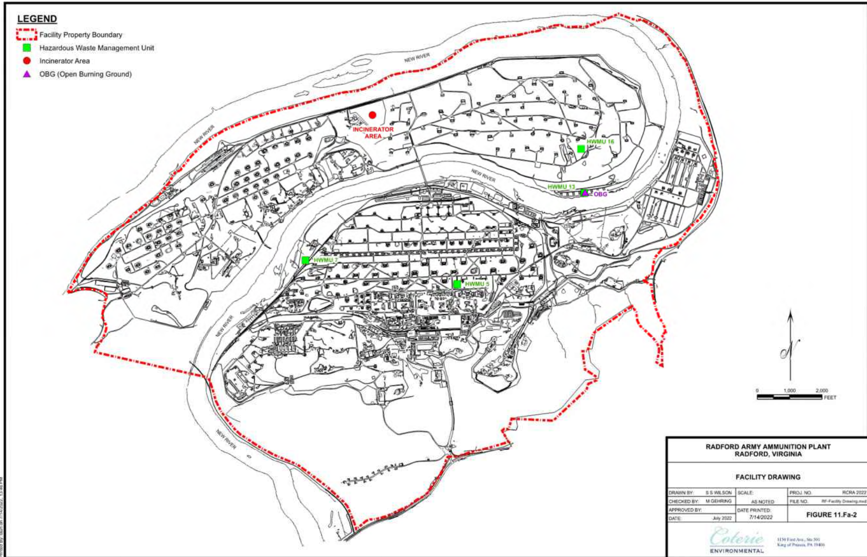
Figure II.Fa-2 – Plot Plan
