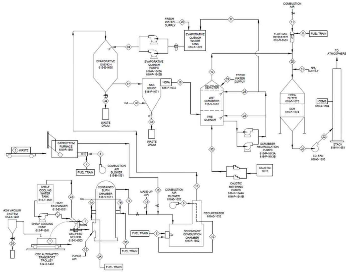
Figure II.Ea-4 - Process Schematic for the CBC and Car Bottom Oven System
