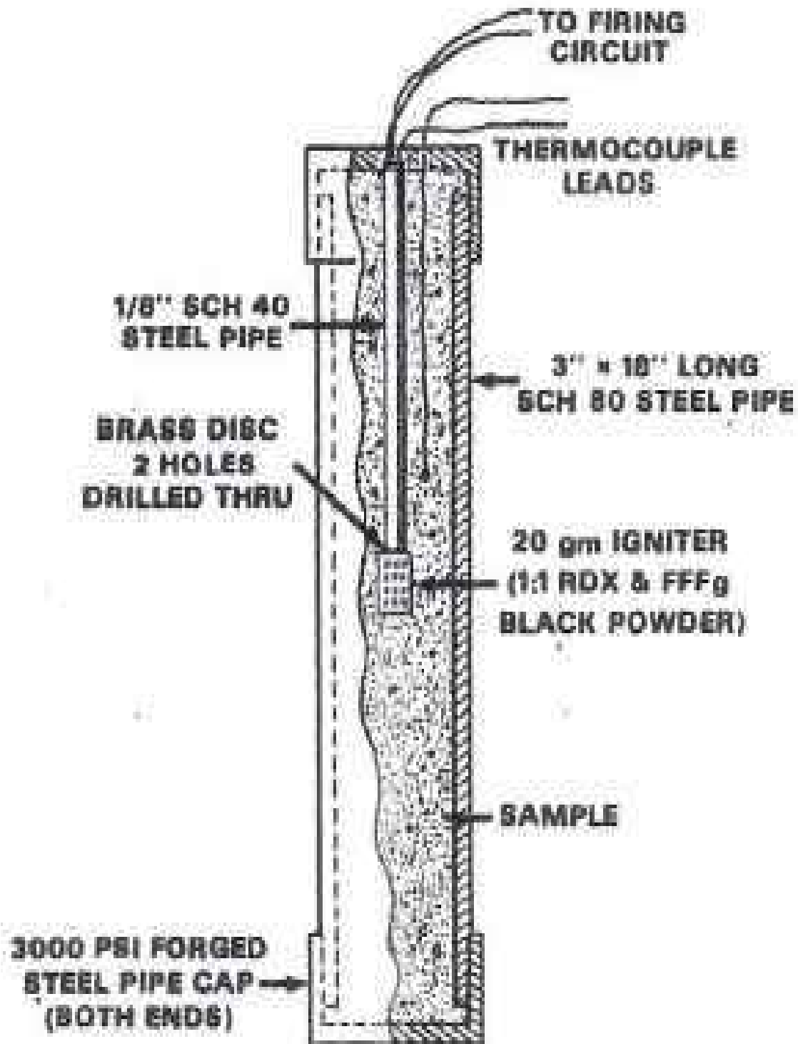
Figure B2. Experimental arrangement for deflagration-detonation transition test Source: Hercules Incorporated (Radford Army Ammunition Plant)
