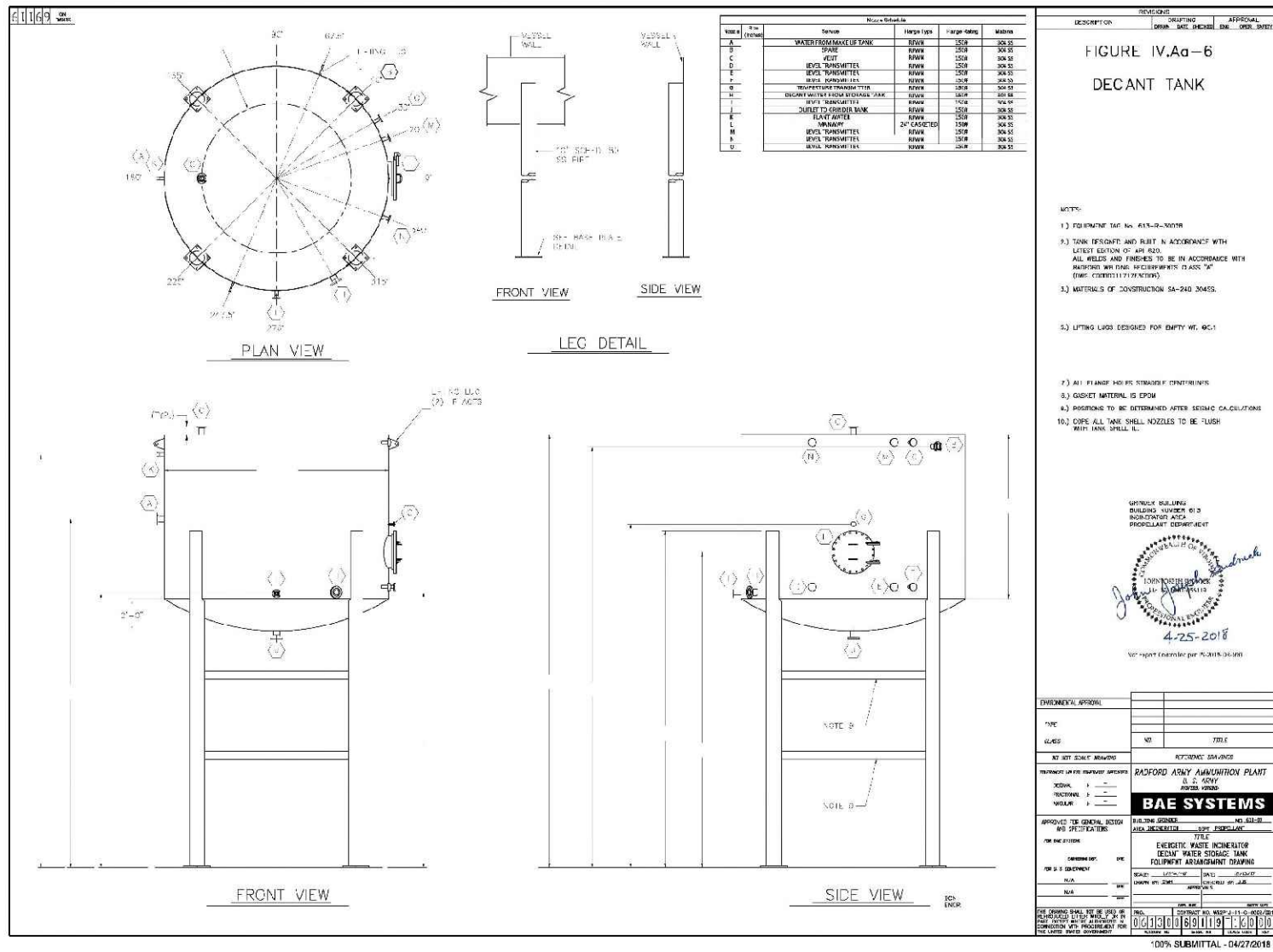
Figure IV.Aa-6 – EWI-CWP Complex Decant Tank Engineering Drawing (DWG No. 061300-69119-T160-00)
