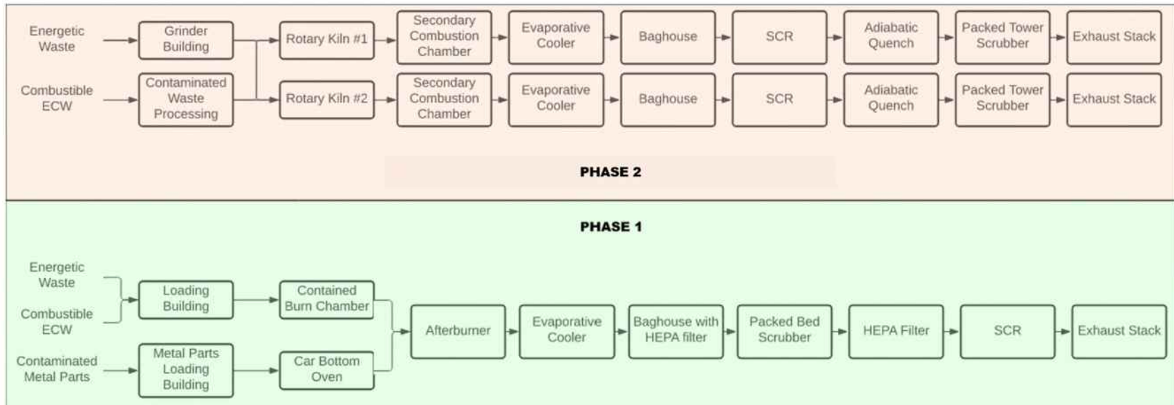
Figure V.Aa-1 – EWI-CWP Process Schematic
