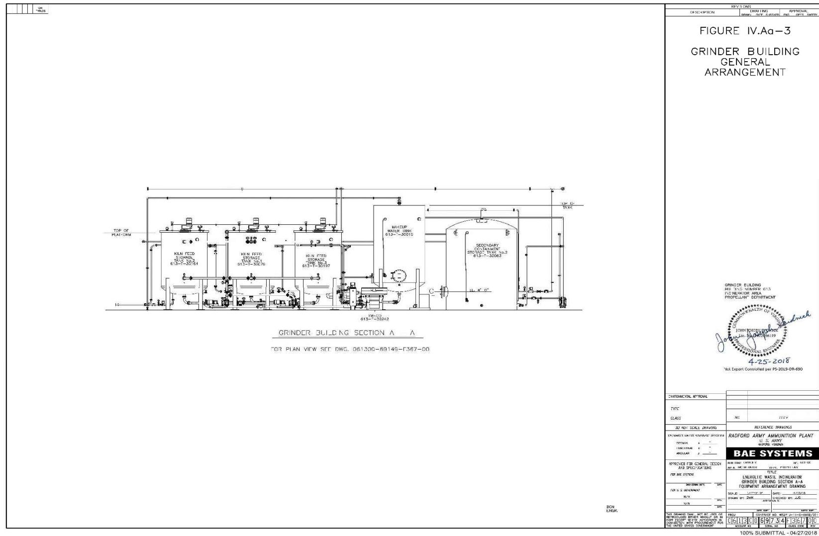
Figure IV.Aa-3 – EWI-CWP Complex Grinder Building General Arrangement Drawing, Elevation A-A (061300-69734-F367)
