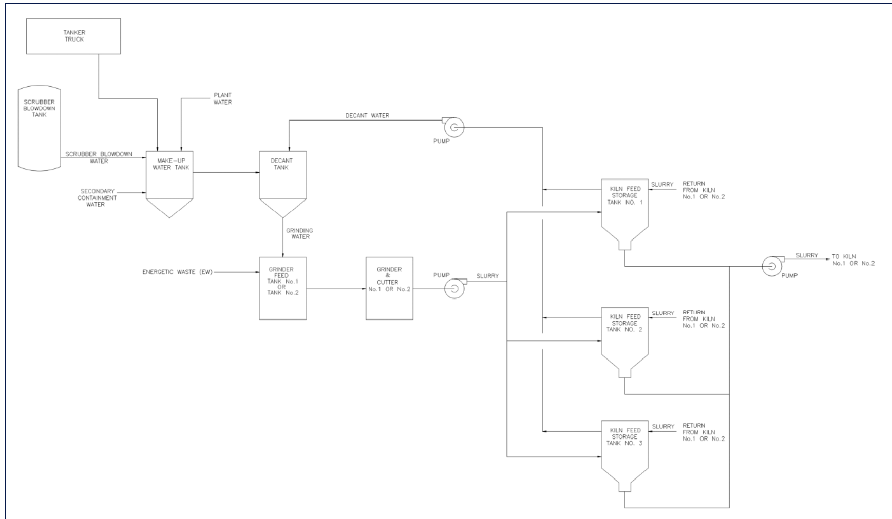
Figure II.Ea-3 – EWI-CWP Grinder Building Process Schematic
