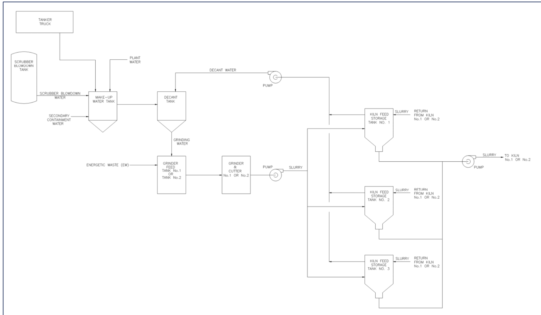
Figure IV.Aa-1 – EWI-CWP Complex Grinder Building General Process Flow
