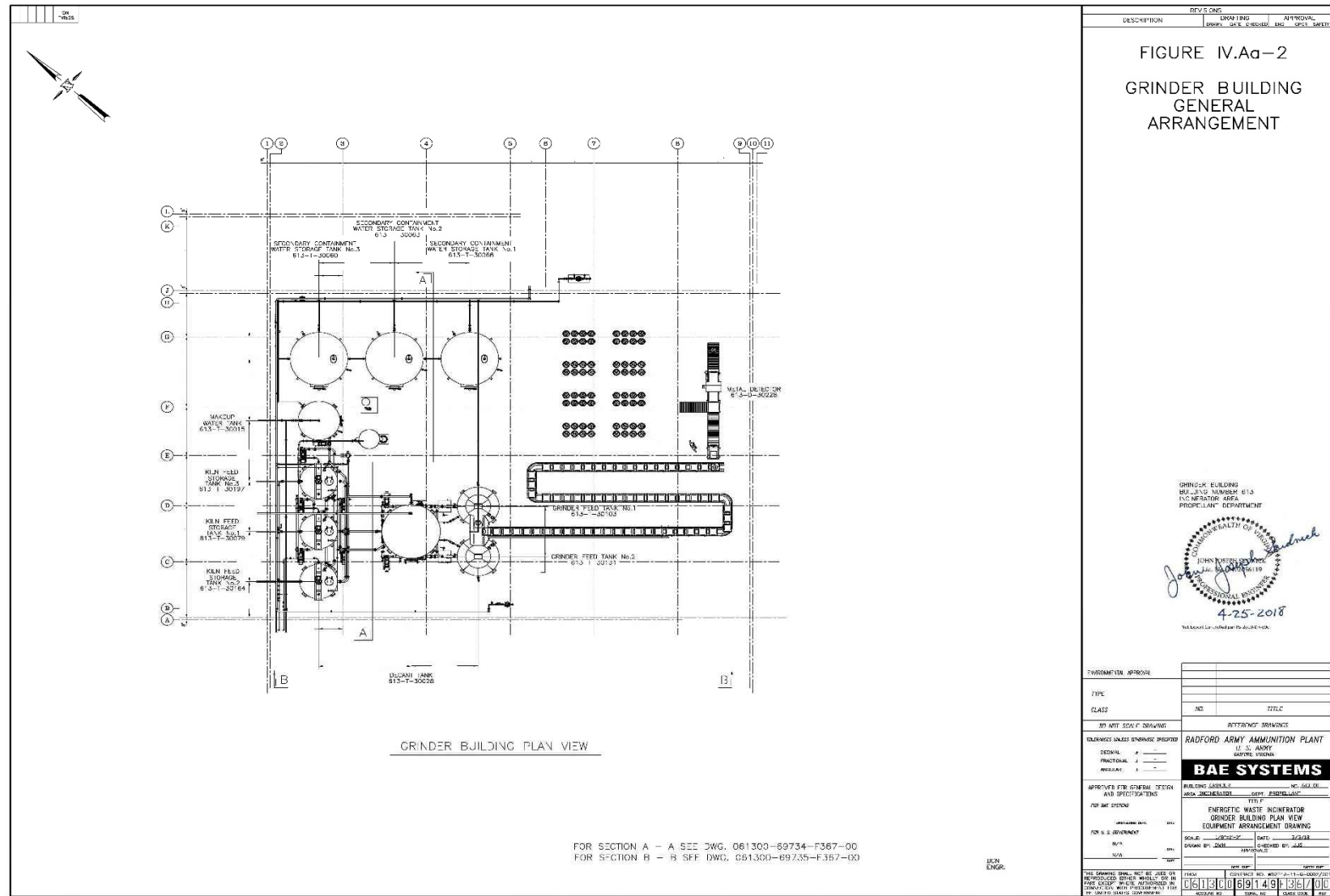
Figure IV.Aa-2 – EWI-CWP Complex Grinder Building General Arrangement Drawing, Plan View (061300-69149-F367)
