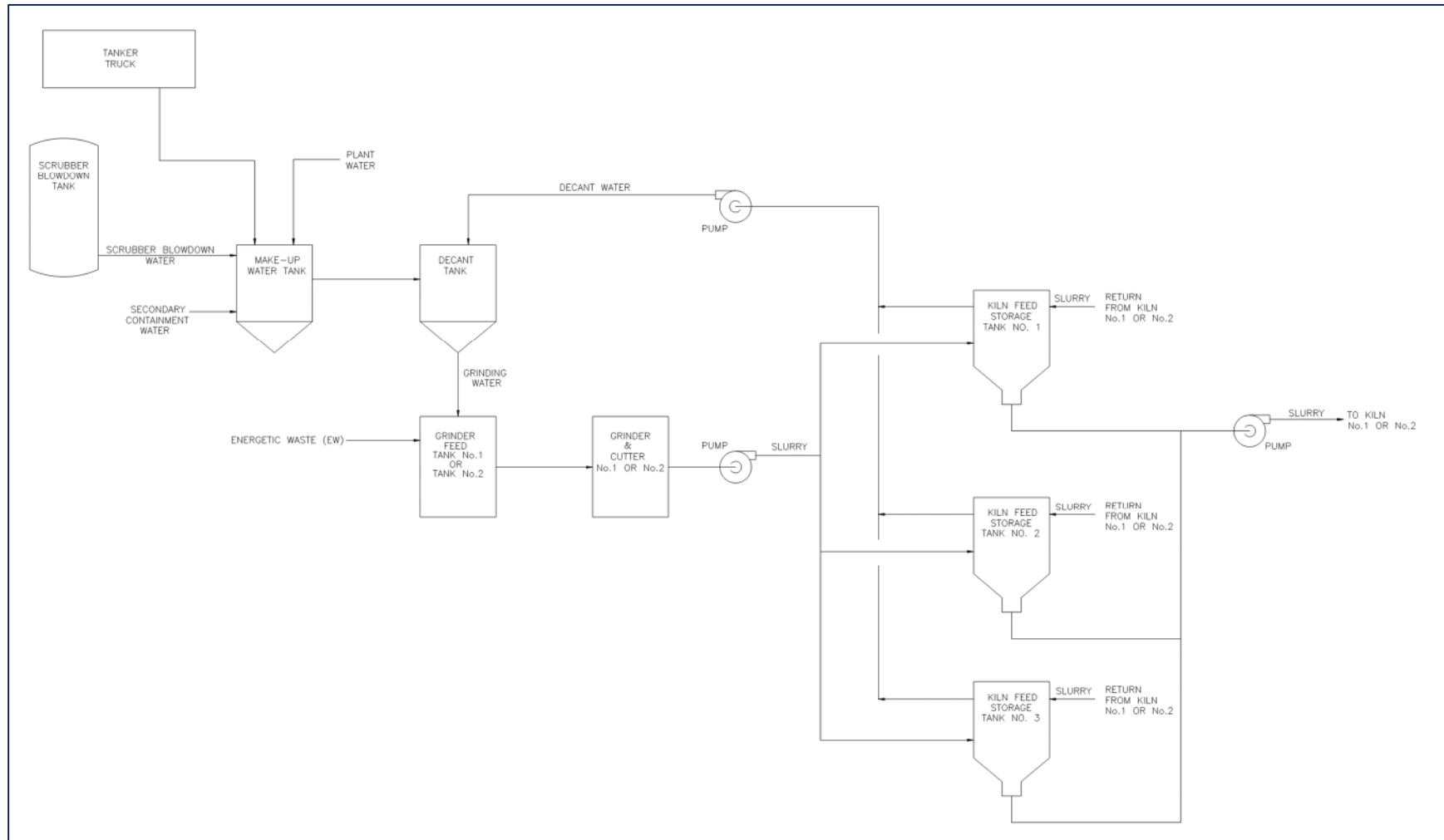
Figure II.Fa-4 – EWI-CWP Grinder Building Process Schematic
