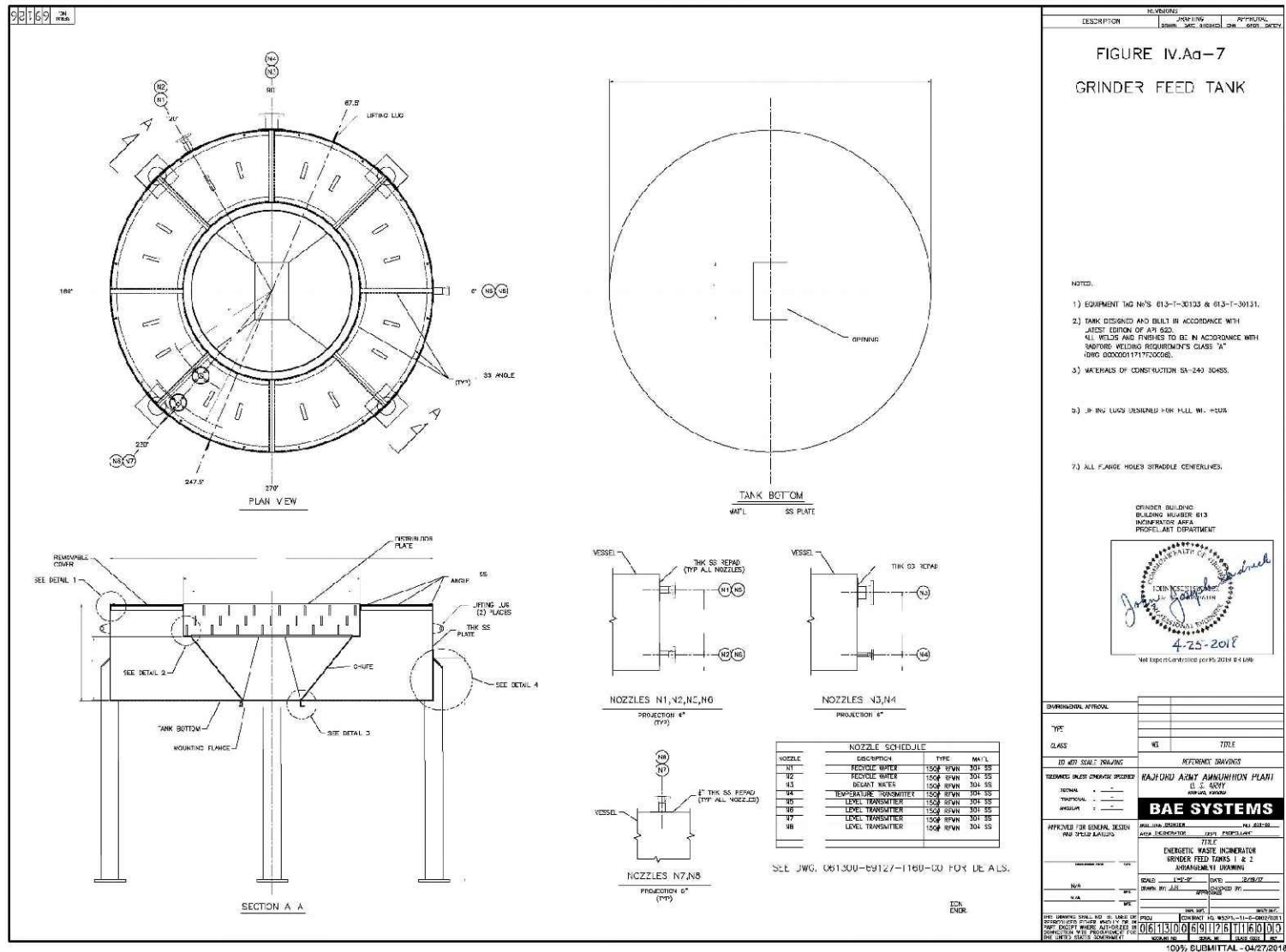
Figure IV.Aa-7 – EWI-CWP Complex Grinder Feed Tank Engineering Drawing (DWG No. 061300-69126-T160-00)
