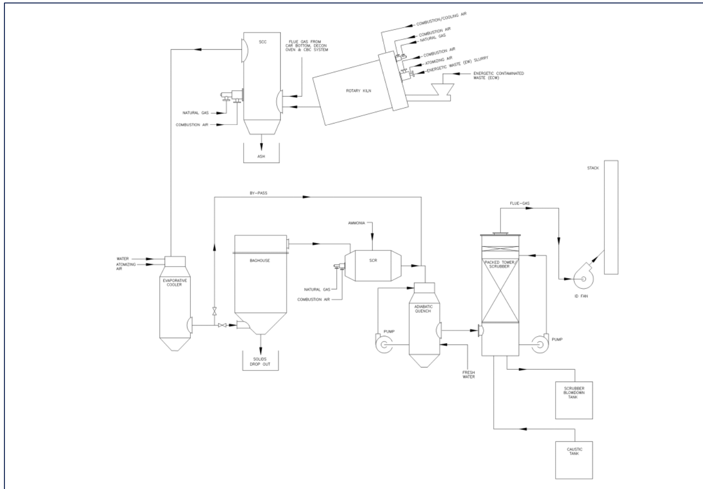
Figure II.Fa-6 - Kiln System Process Schematic (identical for each)
