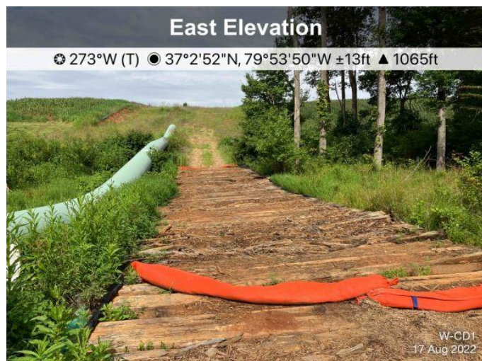
Figure 3: Designated crossing W-CD1, ECD's are in place.
