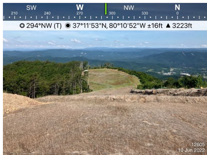
Figure 4: STA 12605+00 – Controls in place and functioning properly. Area stabilized with erosion matting.
