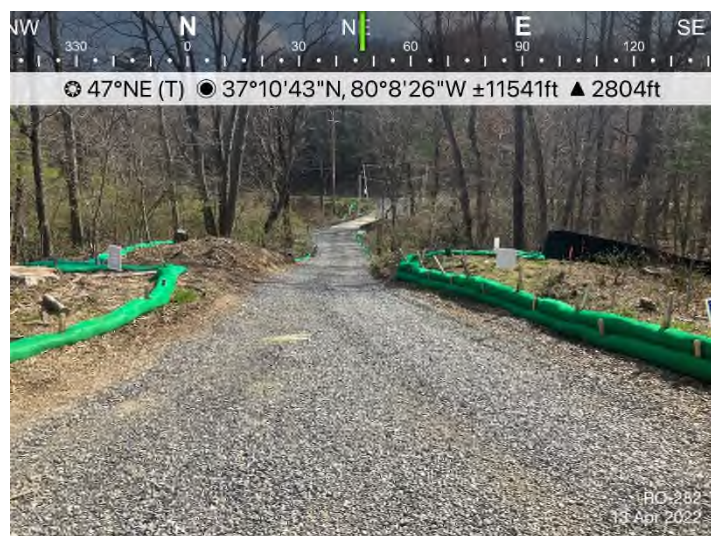
Figure 3: STA 12773+00 – Controls in place and functioning properly. Area stabilized with erosion control matting.
