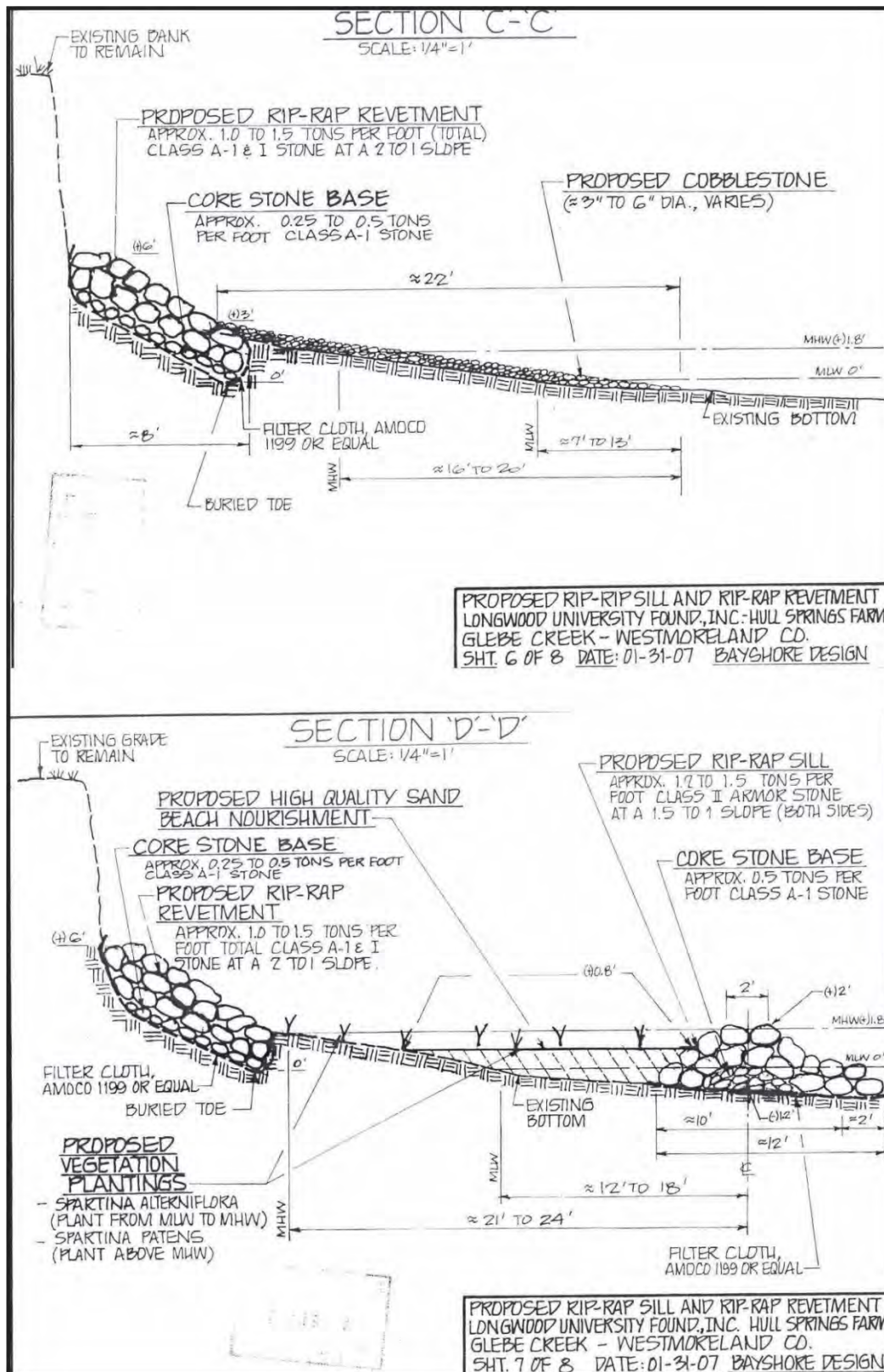
Figure 9-9. Typical cross-sections for the Hull Springs Farm Living Shoreline project. CC shows the cobble gap, and DD shows the revetment at the base of bank as well as the sill. Cross-sections courtesy of Bayshore Design.
