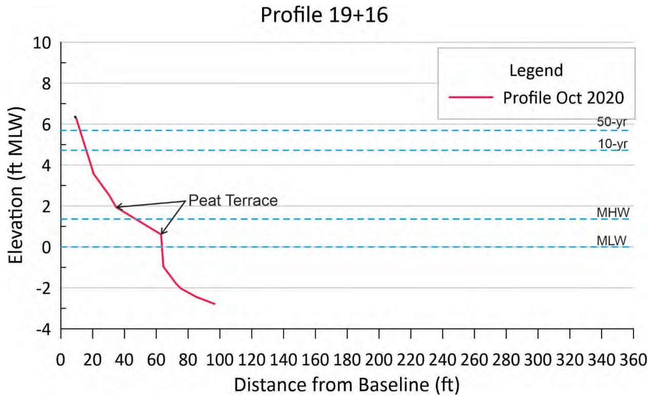
Figure 8-12. Cross-shore profile 19+16 at Haven Beach south of the breakwaters shows the wide peat terrace that occurs.
