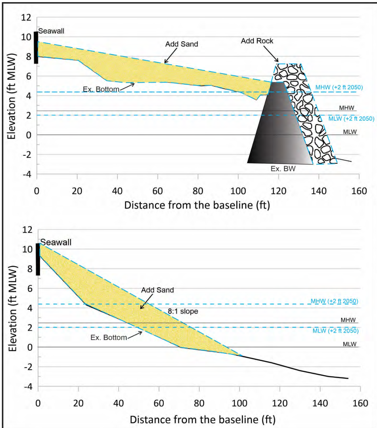
Figure 10-5. Existing conditions at a high bank breakwater site (VIMS East). The land continues to rise behind the seawall and infrastructure exists so the site could not be graded. To raise the elevation of the system to adjust for the projected 2050 tide level (blue) rock can be added to the structures. In addition, sand can be added behind the structures and in the embayments to enhance adaptability. After Hardaway et al., (2019).
