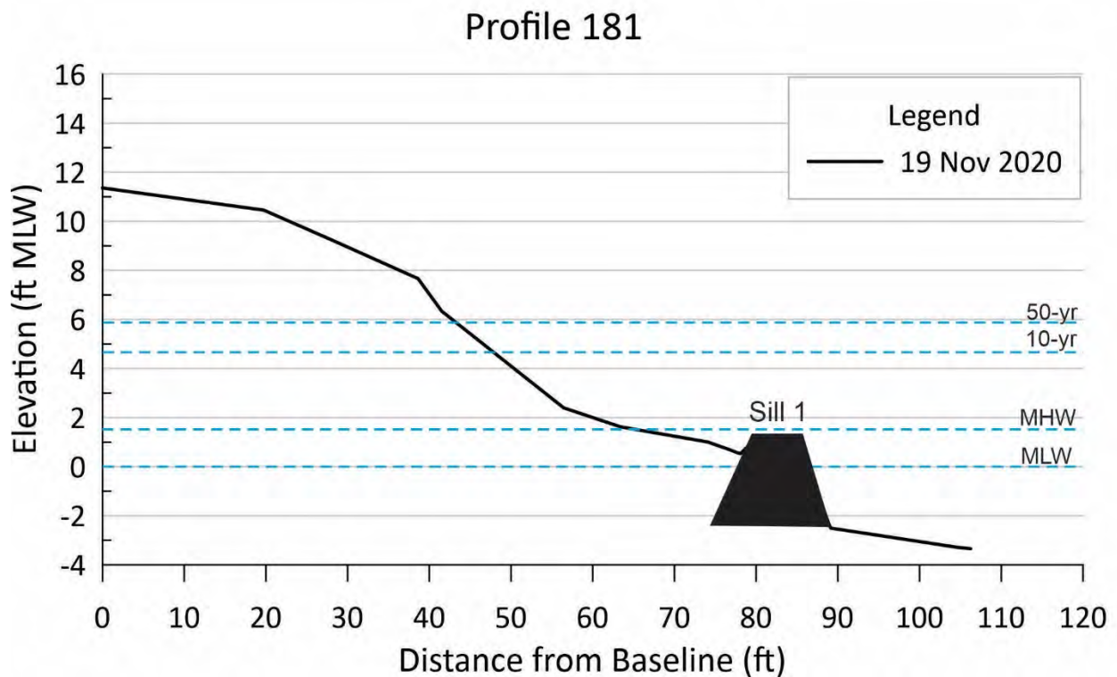
Figure 9-15. Profile cross-sections from Hull Springs Farm taken on 19 November 2020. Profiles 98 and 181 cross Sill 1.
