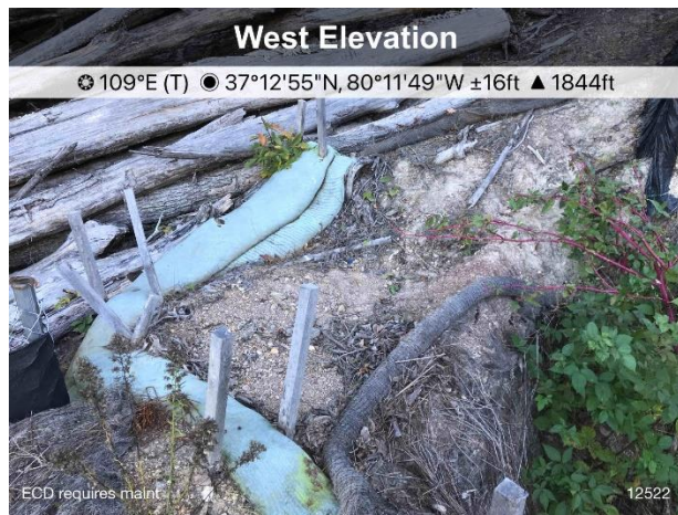
Figure 3: St 12522 CFS requires maintenance
