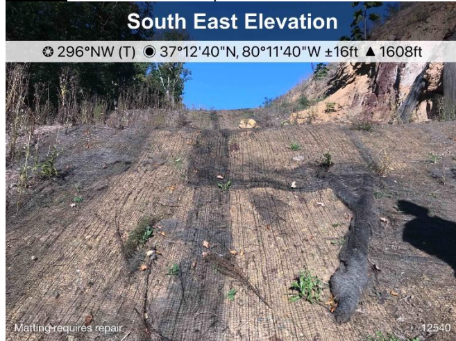
Figure 1: St 12540 ROW requires additional stabilization
