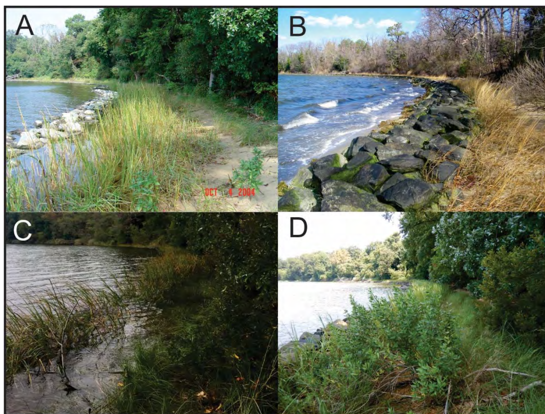
Figure 4-3-4. Photos of St. Mary's A) two years after construction (4 Oct 2004), B) 11 years after construction (1 Feb 2013), C) 15 years after construction (13 Oct 2017), D) 16 years after construction (15 Aug 2018).
