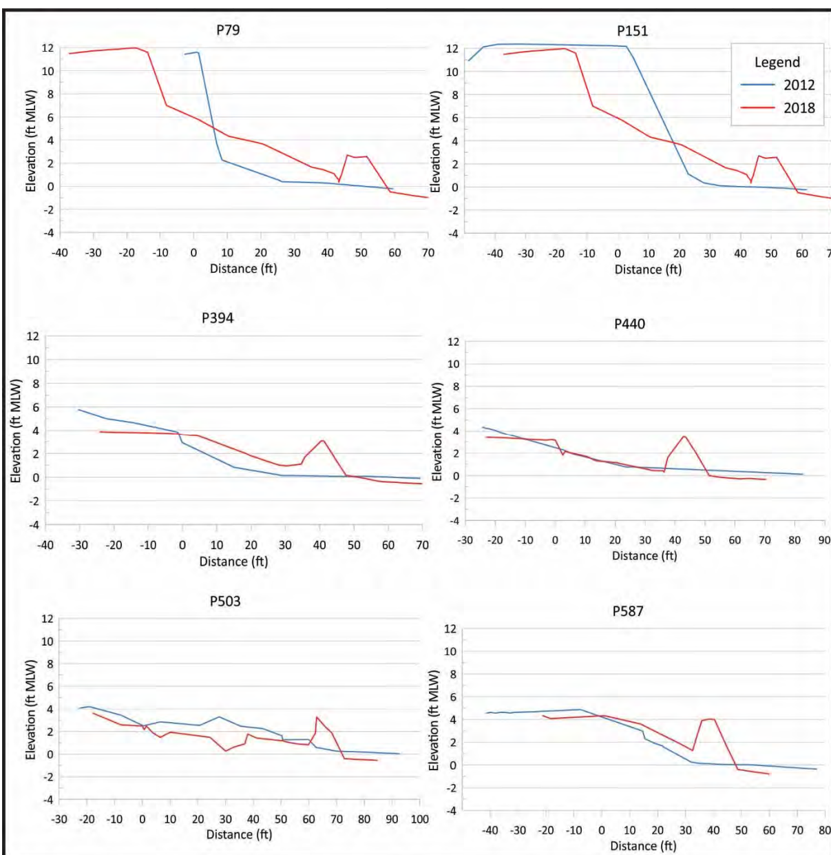
Figure 4-2-8. Cross-sectional profiles at Occohannock taken before the living shoreline project was installed and in 2018.
