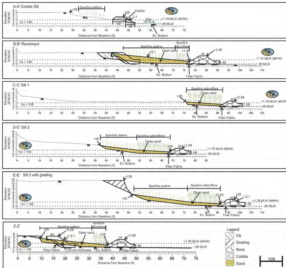
Figure 4-2-3. Typical cross-sections for Camp Occhohannock living shoreline.
