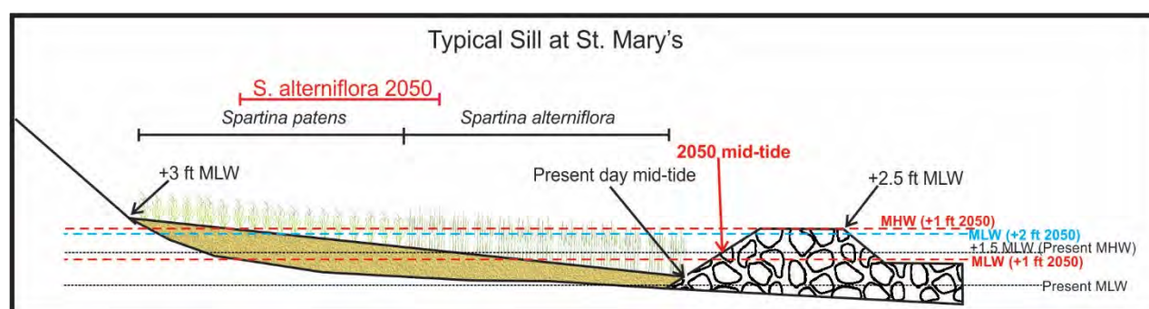
Figure 5-3-1. Sea-level rise scenarios modeled at St. Mary's and depicted on a typical cross-section.
