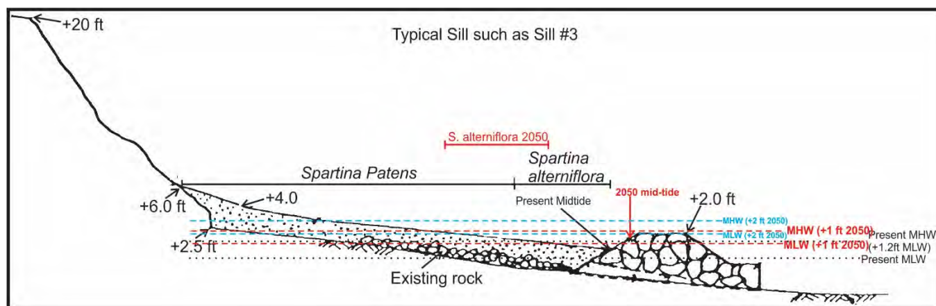
Figure 5-4-1. Sea-level rise scenarios modeled at Jefferson Patterson and depicted on a typical cross-section.
