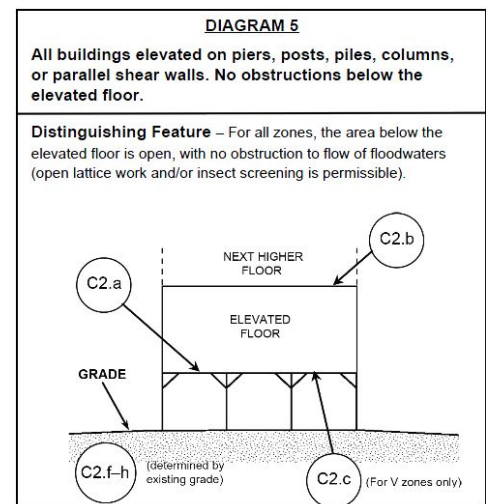
Figure 9: Building diagram for structure elevated on piers, posts, piles, columns, or parallel shear walls.
