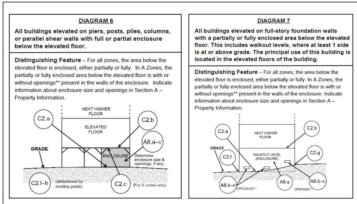
Figure 6: FEMA (2015) building diagram for structures elevated on partial or full enclosures at grade (Diagram 6) or partially below grade (Diagram 7).
